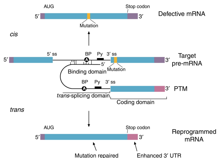
Figure 6 The anatomy of a PTM. The figure depicts a mutant target pre-mRNA (see the LacZ model system in ref. 12) that is incapable of coding for functional protein because it contains a mutation in the second exon (indicated as orange segment). The product of the conventional cis -splicing reaction for this pre-mRNA is a defective mRNA. The PTM shown contains several domains. The binding domain (also referred to as the targeting domain) binds to the pre-mRNA target, thus localizing the PTM near the site of the desired trans -splicing reaction. The binding domain can also be designed to occlude important elements within the 3' splice site of the target and thus reduce the cis -splicing reaction. Between the binding domain and the trans -splicing domain there is usually a spacer region for flexibility. The trans -splicing domain, which in the case shown includes the elements required to make a potent 3' splice site, is responsible for the reactivity of the PTM. Finally, the coding domain contains the necessary genetic information that will be imparted into the reprogrammed RNA. This can include protein-coding instructions as well as instructions for the effective processing, transport, and localization of the reprogrammed mRNA. In the example shown, the open reading frame has been changed to repair the mutation in the gene, and the 3' untranslated region (3' UTR) has been enhanced to increase mRNA stability and translation. It should be noted that the cis - and trans -splicing reactions are in competition. This implies that as the level of reprogrammed mRNA increases, the level of defective mRNA decreases. A decrease in the level of defective mRNA may be very useful in the case of dominant mutations.
